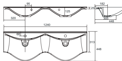
DOUBLE BOWL
