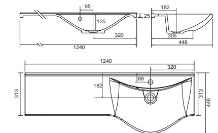
RH BOWL
