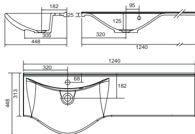
LH BOWL
