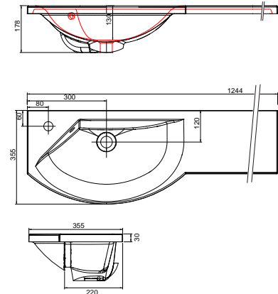
ART 1244MM LH SLIMLINE
