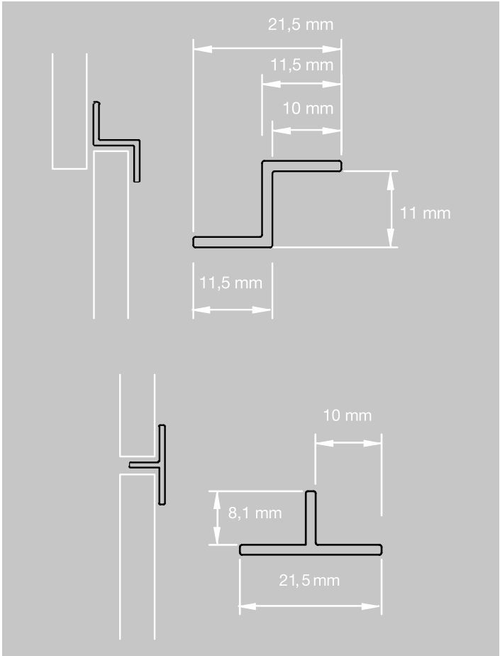
Z and T shaped profile (White/Chrome)
