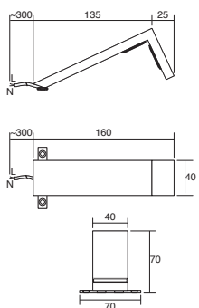
ARAL 3923 £109.20 W40 x D160 x H70 mm 2x1.2W • Transformer Included • IP21
